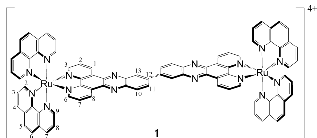
Scheme 1. Chemical structure of 1 , the \Delta,\Delta enantiomer of [\mu-(\text{bidppz})-(\text{phen})_2\text{Ru}_2]^{4+} ; phen = 1,10-phenanthroline, bidppz = 11,11'-bis-(dipyrido[3,2- a :2',3'- c ]phenazinyl).
